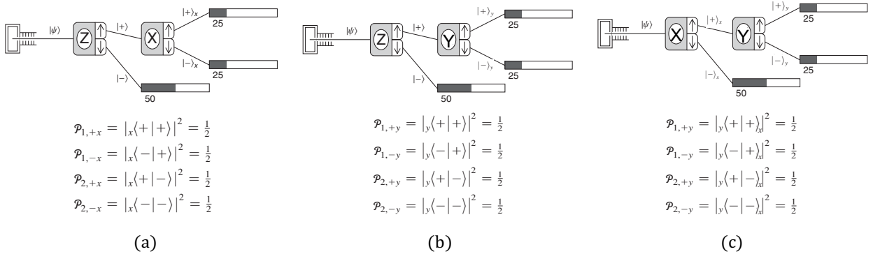
FIG. 4. Different configurations of sequential SG experiments are treated formally in order to motivate the need for complex numbers for the description of quantum state vectors. j_x h+j+i j^2 = \frac{1}{2} represents the probability that the output state is j+i_x when the input state is j+i . Figures adapted from Ref. 19.
