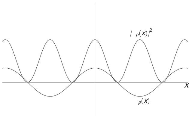
FIG. 1. Graphs of \psi_p(x) = A \cos \frac{p x}{\hbar} and |\psi_p(x)|^2 . The graph of |\psi_p(x)|^2 (probability distribution) is inconsistent with the assertion that once momentum is exactly determined, one should have no information about the electron's position.
