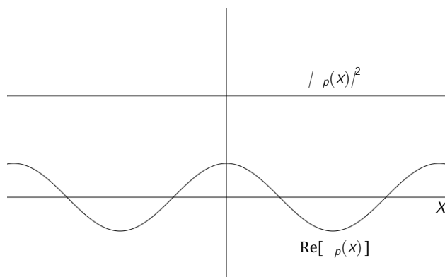
FIG. 2. Graphs of \text{Re}[\psi_p(x)] and j\psi_p(x)j^2 for \psi_p(x) = Ae^{\frac{ipx}{\hbar}} . Now the contradiction is eliminated, since there is no information about the electron’s position for a state of definite momentum.
